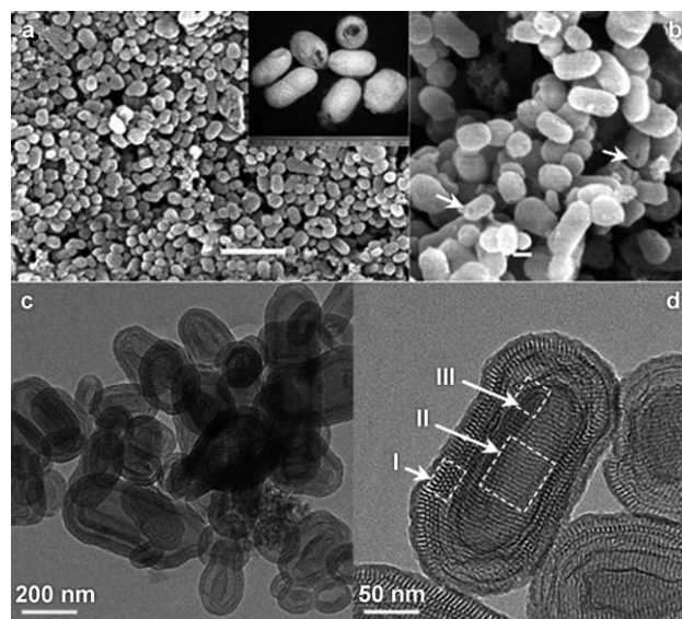
Figure 1. SEM images (a,b) and TEM images (c,d) of calcined nanopods. Scale bar is 1 \mu m in (a) and 100 nm in (b). The inset of (a) is a digital camera image of silkworm cocoons. The white arrows in (b) show partially broken particles (see the main text).
